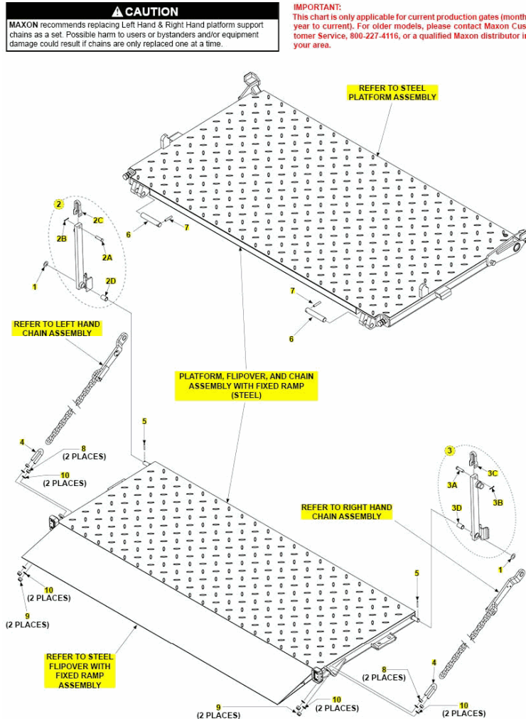
PLATFORM, FLIPOVER, AND CHAIN ASSEMBLY WITH FIXED RAMP (STEEL)
