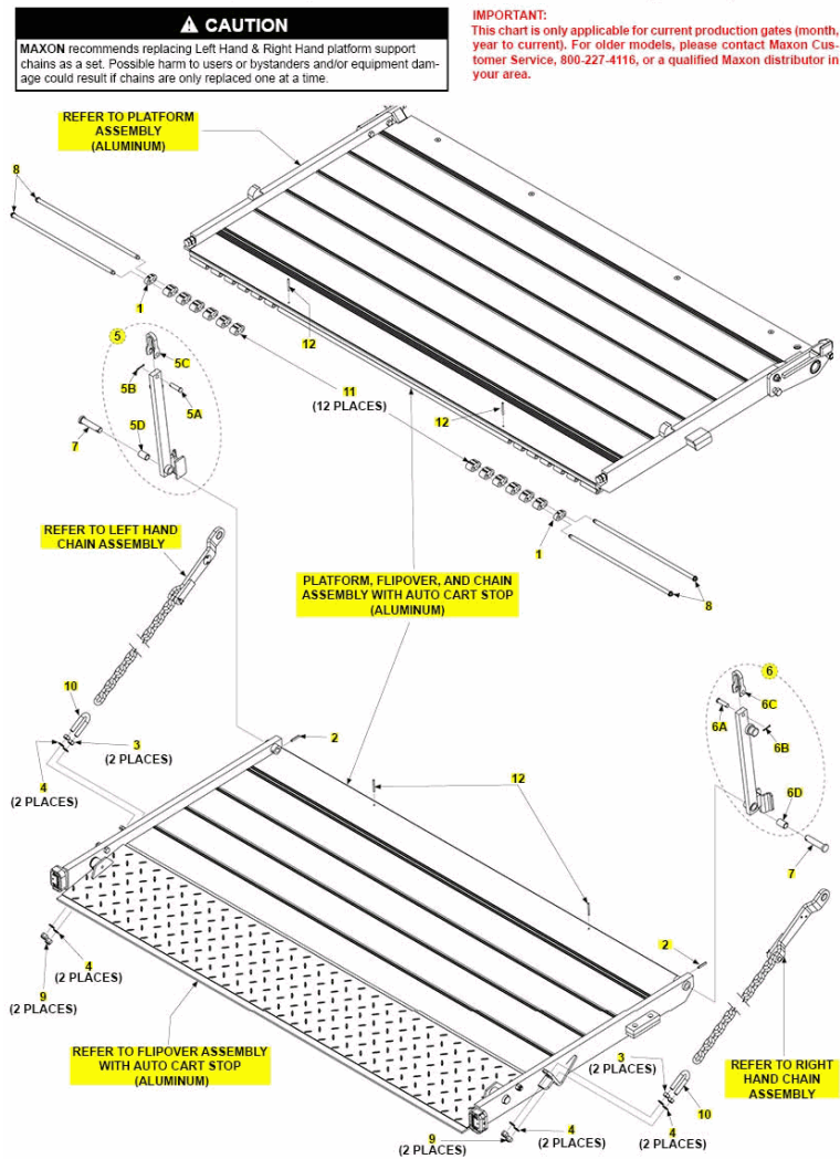
PLATFORM, FLIPOVER, AND CHAIN ASSEMBLY WITH AUTO CART STOP (ALUMINUM)
