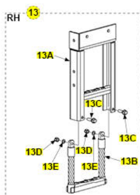
FLEXIBLE STEP ASSEMBLY WITH NO RUBBER BUMPER
