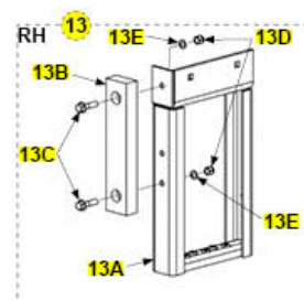
SINGLE STEP ASSEMBLY WITH PLASTIC BUMPER
