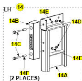
SINGLE NO STEP ASSEMBLY WITH BUMPER
