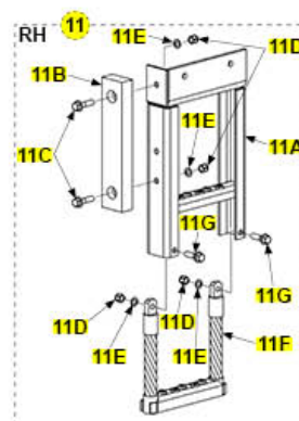
FLEXIBLE STEP ASSEMBLY WITH PLASTIC BUMPER
