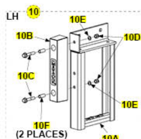
SINGLE STEP ASSEMBLY WITH RUBBER BUMPER
