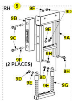
FLEXIBLE STEP ASSEMBLY WITH RUBBER BUMPER
