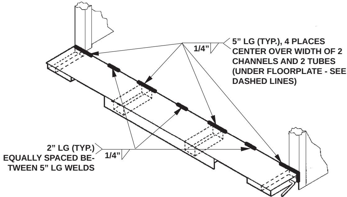
EXTENSION PLATE WELDS - VIEWED FROM ABOVE FIG. 9-1
