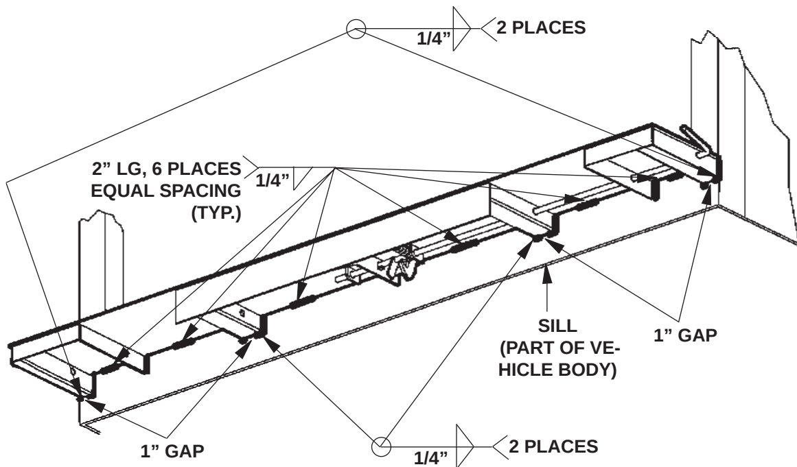
EXTENSION PLATE WELDS - VIEWED FROM ABOVE FIG. 9-1
