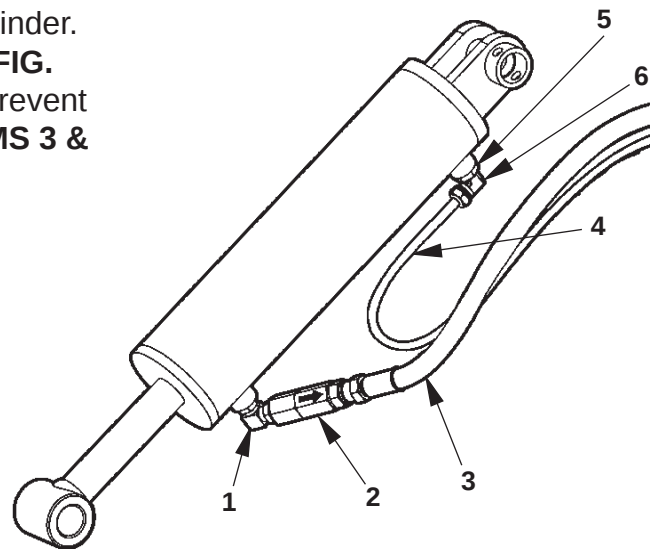
HOSE & TUBING RUN TO HYDRAULIC CYLINDER FIG. 15-2
