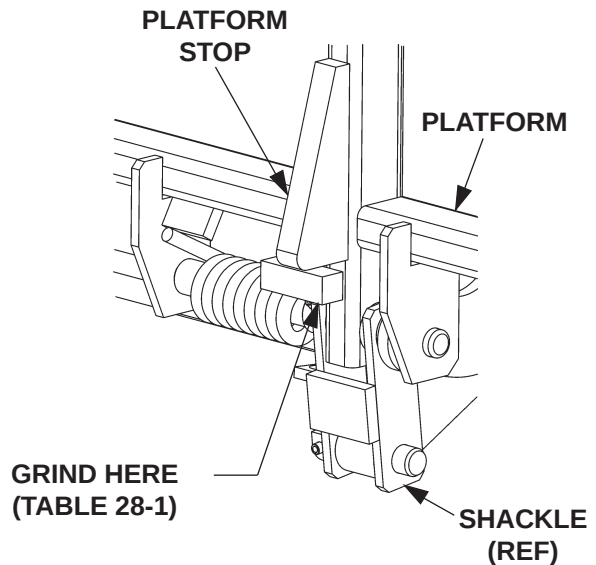
GRINDING PLATFORM STOPS (CURBSIDE SHOWN) FIG. 28-2
