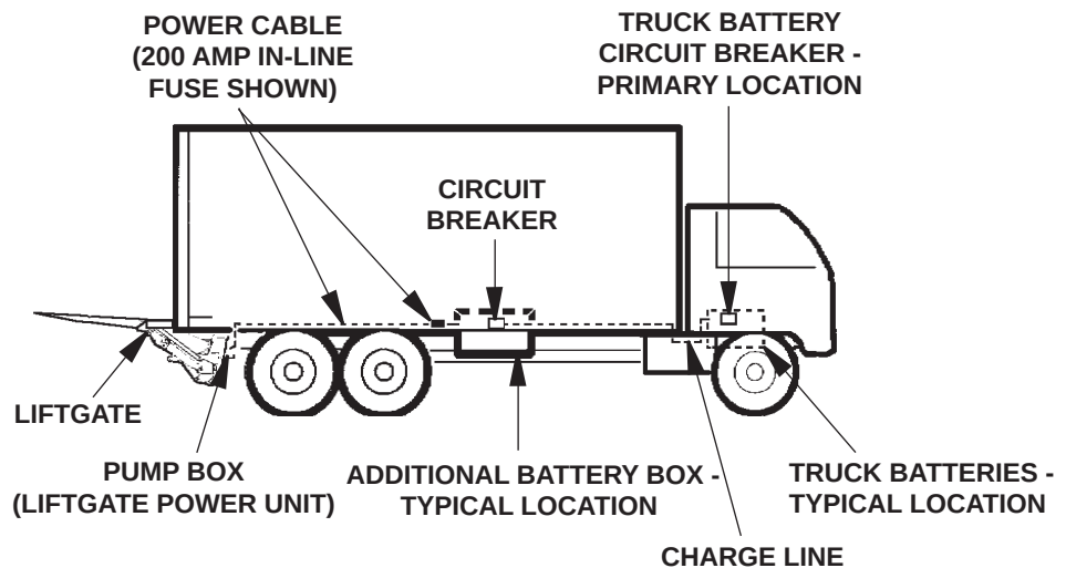
RECOMMENDED LIFTGATE & BATTERY BOX INSTALLATION ON TRAILER FIG. 40-2
