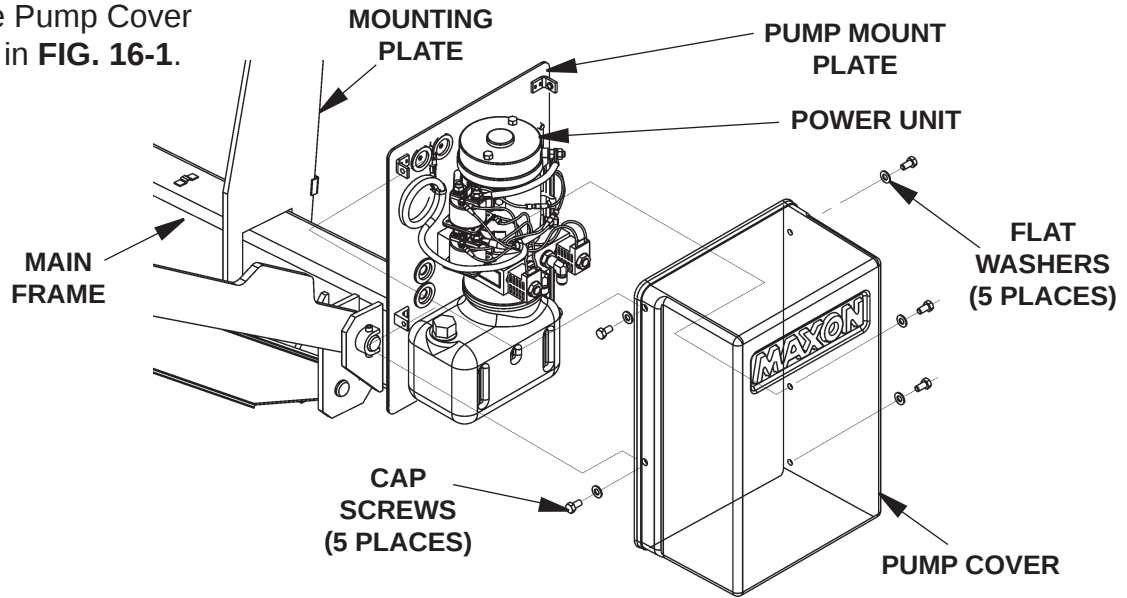
UNBOLTING PUMP BOX COVER FIG. 16-1
