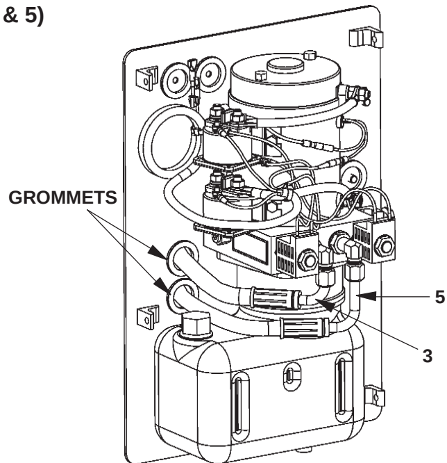
HOSES RUN FROM POWER UNIT FIG. 17-1
