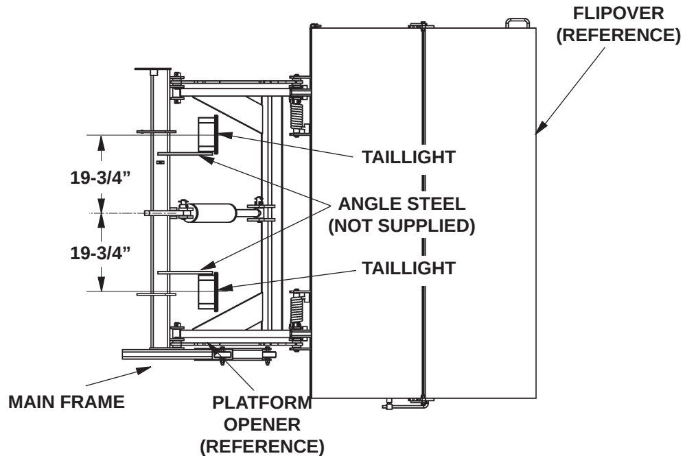
LIFTGATE TOP VIEW FIG. 34-1
