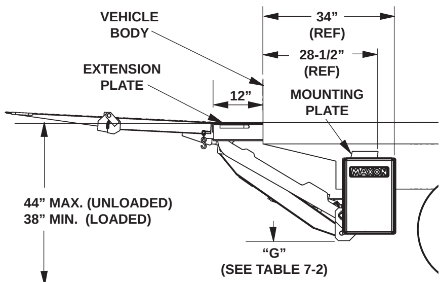
CLEARANCES FOR TE-25L FIG. 7-2
