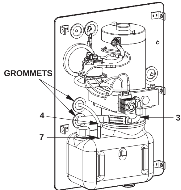
HOSES RUN FROM POWER UNIT FIG. 15-1
