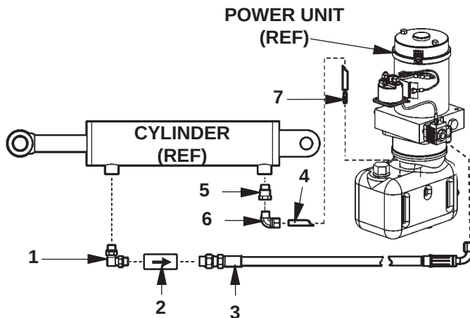
HYDRAULIC SYSTEM PARTS FIG. 14-2
