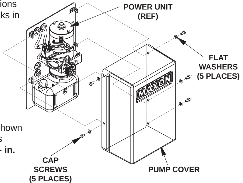
BOLTING ON PUMP COVER FIG. 26-1
