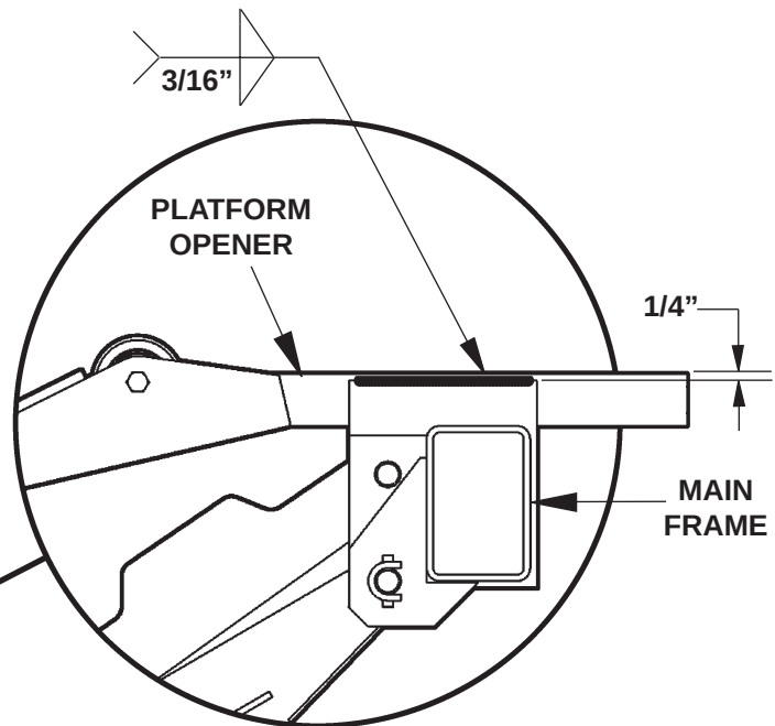
WELDING THE OPENER (VIEW FROM INBOARD SIDE) FIG. 30-1B
