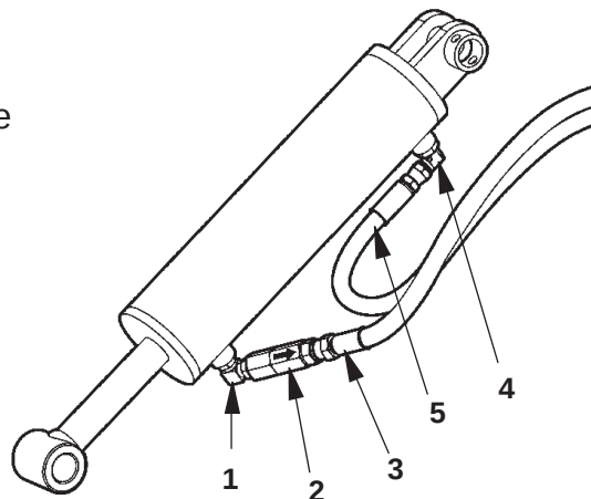
HOSES RUN TO HYDRAULIC CYLINDER FIG. 17-2
