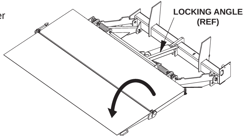
PLATFORM & FLIPOVER UNFOLDED FIG. 12-1
