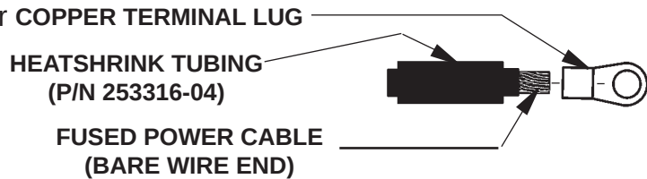
PLACING TERMINAL LUG & HEATSHRINK TUBING ON FUSED POWER CABLE FIG. 20-1
