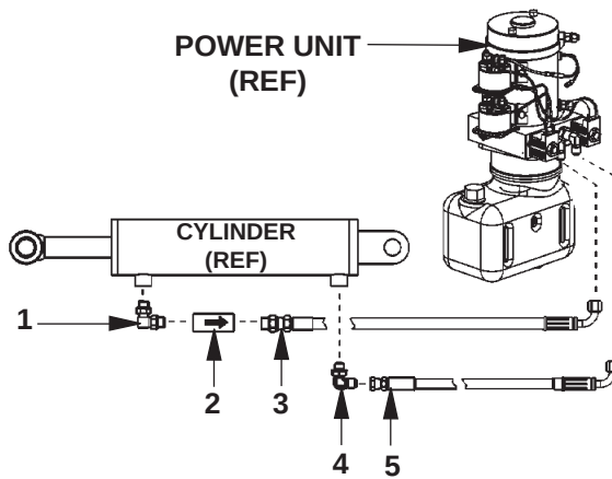
HYDRAULIC SYSTEM PARTS FIG. 16-2
