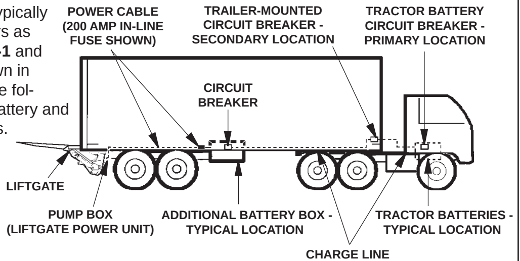
RECOMMENDED LIFTGATE & BATTERY BOX INSTALLATION ON TRAILER FIG. 40-1
