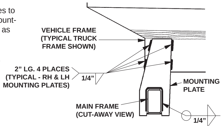
WELD TO VEHICLE FRAME AND MAIN FRAME (RH SIDE SHOWN) FIG. 13-2
