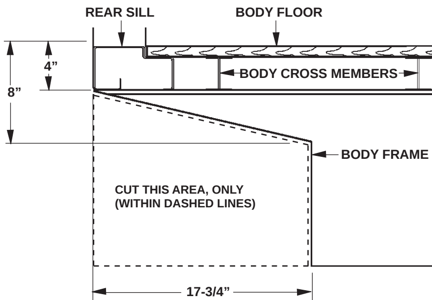
VEHICLE FRAME CUT FOR TE-25L FIG. 8-2
