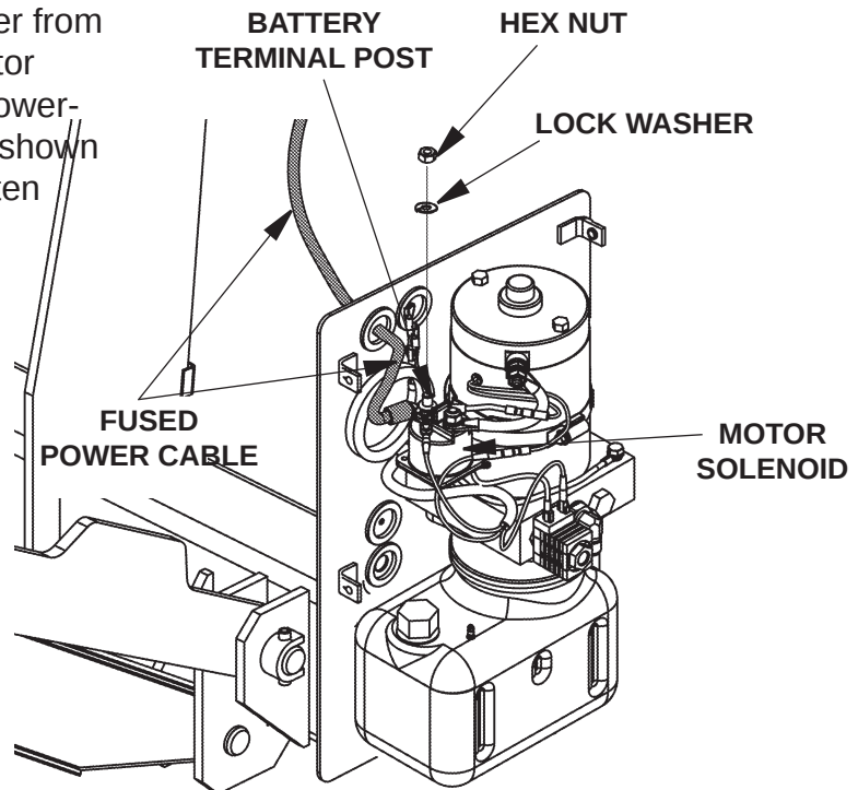
TYPICAL FUSED POWER CABLE CONNECTION (GRAVITY DOWN PUMP SHOWN, HYDRAULIC HOSES NOT SHOWN) FIG. 20-3
