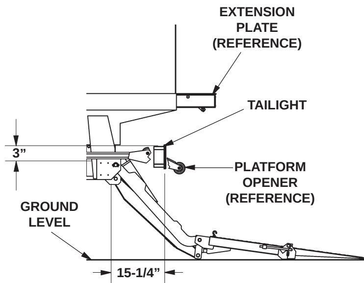
LIFTGATE SIDE VIEW - LEFT HAND SIDE SHOWN FIG. 34-2
