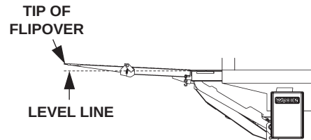
PLATFORM EDGE ABOVE BED LEVEL FIG. 27-2
