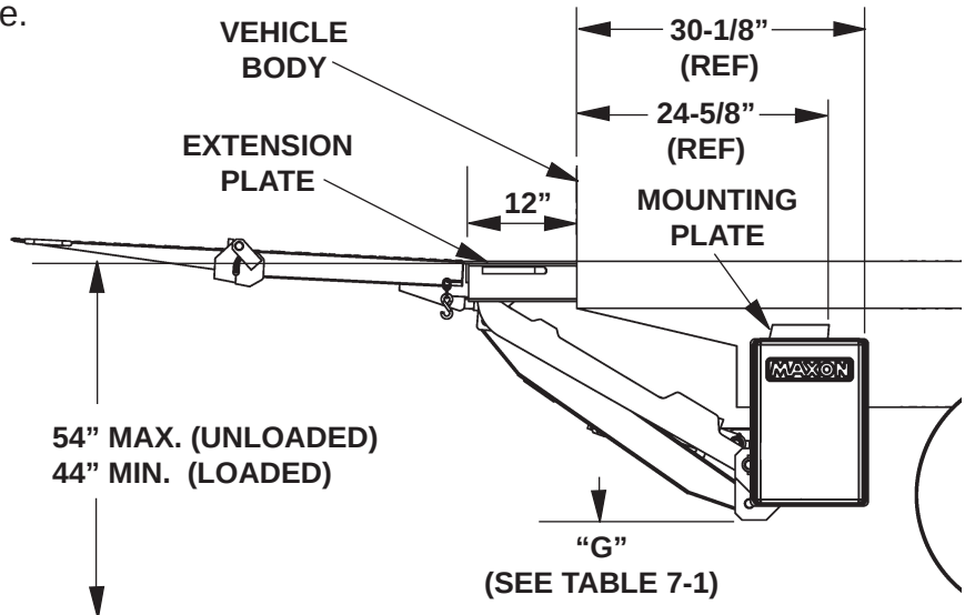
CLEARANCES FOR TE-25 FIG. 7-1
