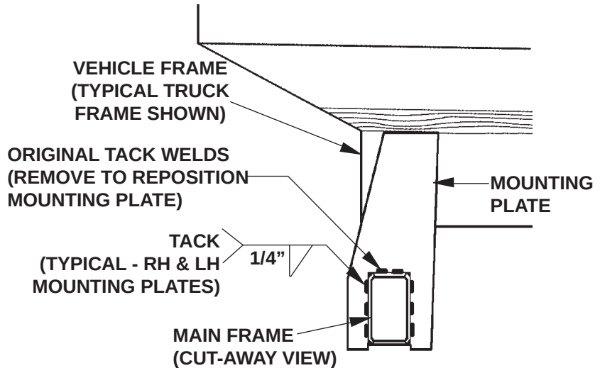
REPOSITIONING MOUNTING PLATE (RH SIDE SHOWN) FIG. 13-1
