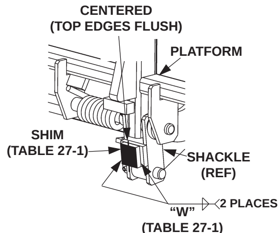
WELDING SHIMS (CURBSIDE SHOWN) FIG. 27-4
