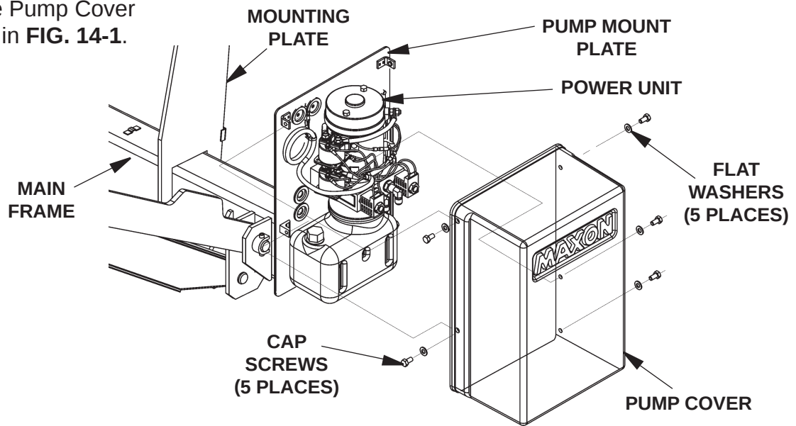
UNBOLTING PUMP BOX COVER FIG. 14-1
