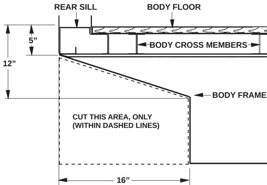
VEHICLE FRAME CUT FOR TE-25 FIG. 8-1
