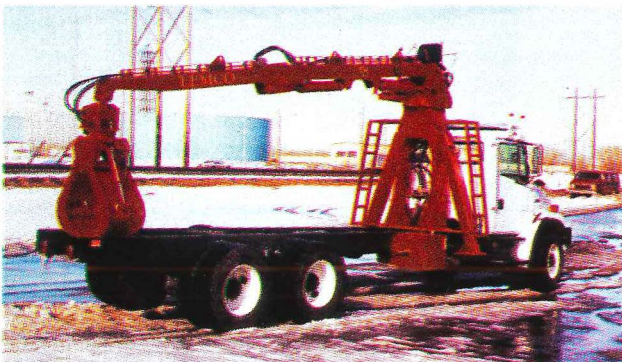
Loaders can be mounted by LEMCO or by local dealer. Knapheide Truck Equipment Company provides sales and service on the Lemco loaders owned by the city of Kansas City.
